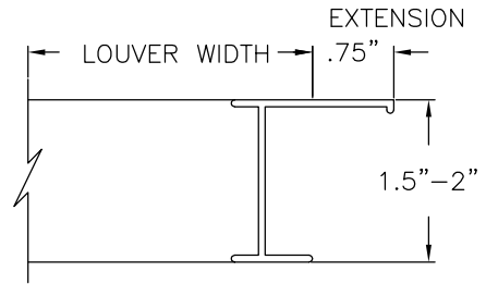
1 1/2" OR 2" DEEP LOUVER
