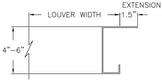
4" OR 6" DEEP LOUVER
