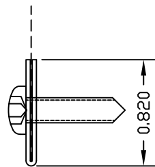
DETAIL "B" SCREEN FRAME
