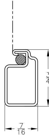
SCREEN FRAME DETAIL
