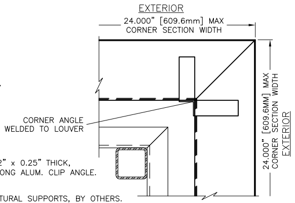
OPTIONAL MITERED CORNER
