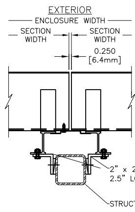
ALTERNATE VERTICAL MULLION AT SUPPORT
