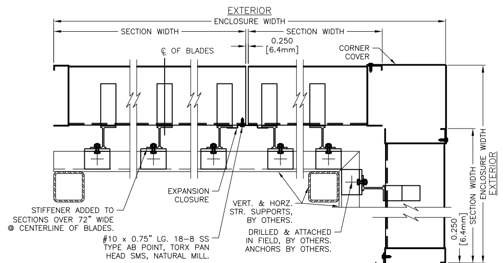
HORIZONTAL SECTION
