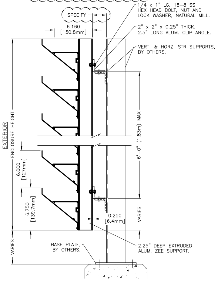
VERTICAL SECTION
