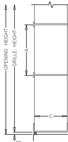
VERTICAL SECTION
