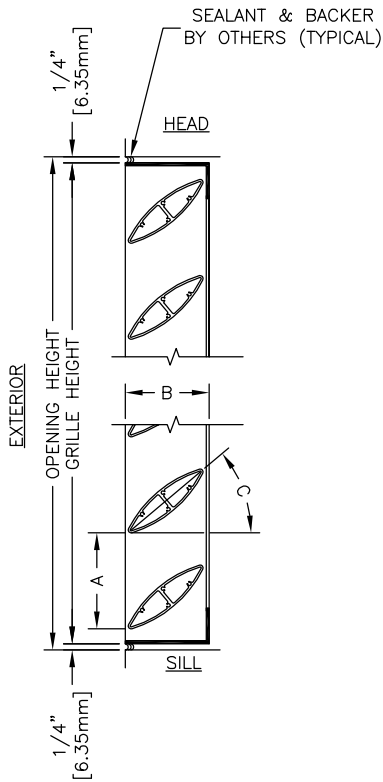
VERTICAL SECTION
