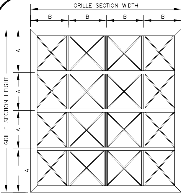
EXTERIOR ELEVATION
