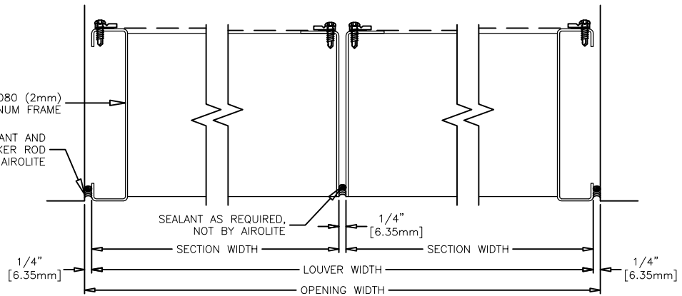
CONCEALED VERTICAL MULLION
