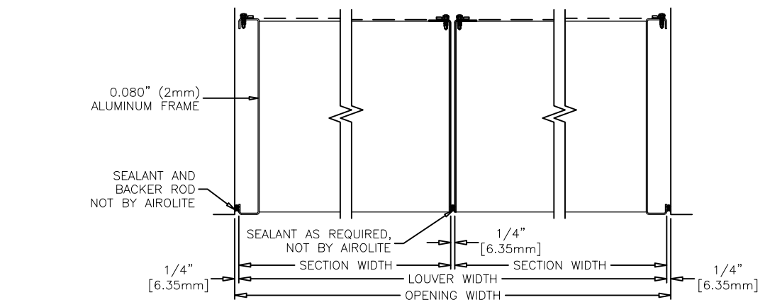
CONCEALED VERTICAL MULLION
