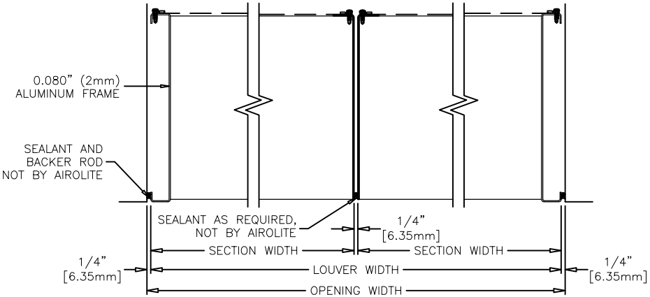
CONCEALED VERTICAL MULLION
