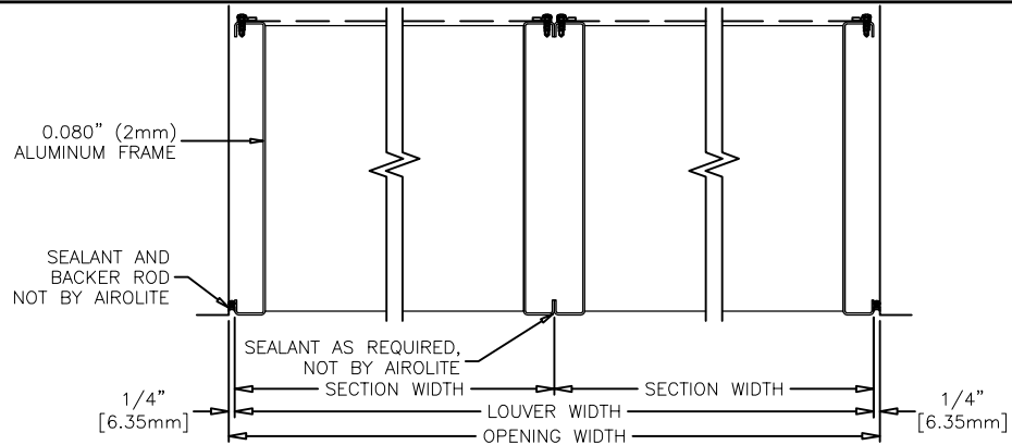
VISIBLE VERTICAL MULLION
