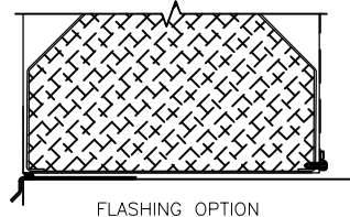
CONCEALED VERTICAL MULLION
