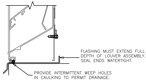
FLASHING OPTION
