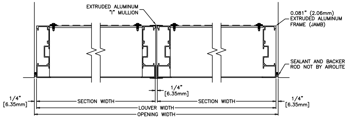
VISIBLE VERTICAL MULLION
