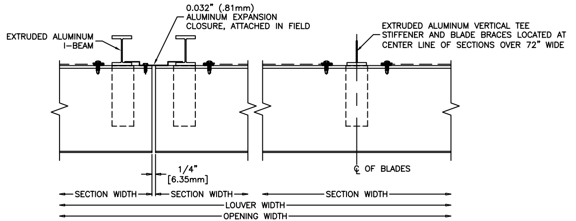
CONCEALED VERTICAL MULLION
