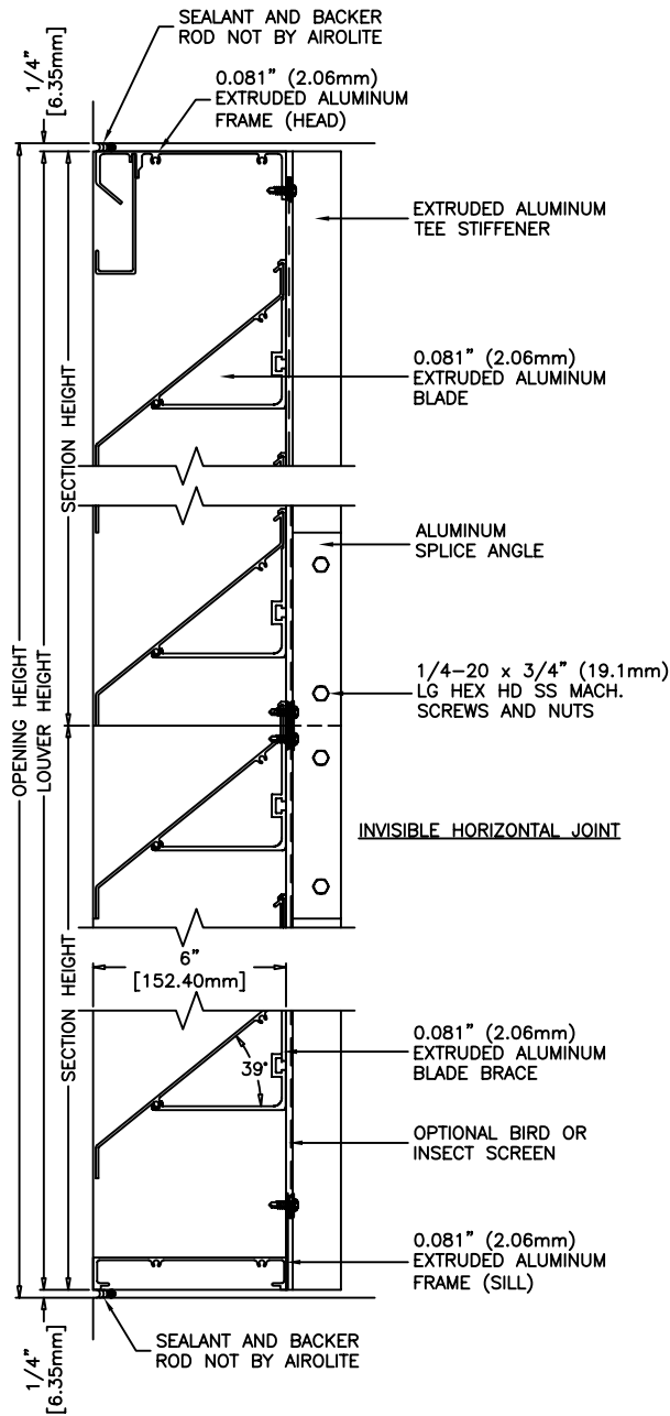
VERTICAL SECTION
