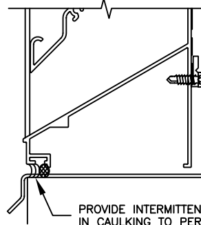
FLASHING OPTION
