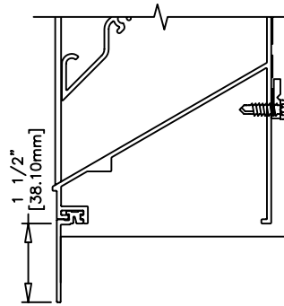
FLANGE OPTION
