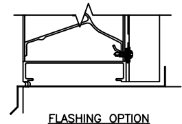
FLASHING OPTION
