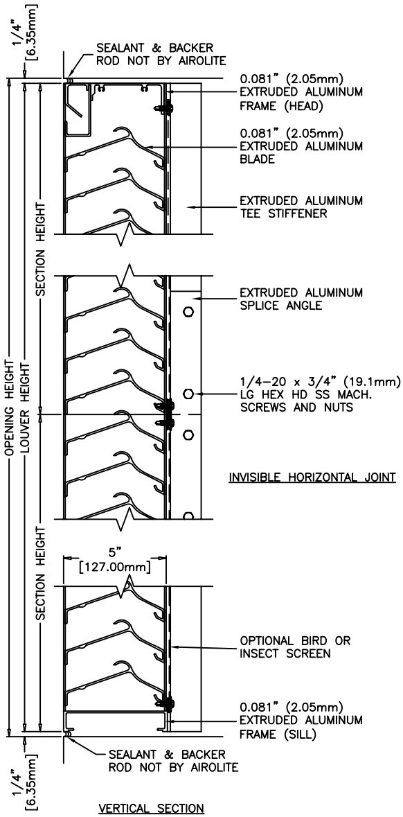
VERTICAL SECTION
