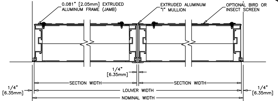
VISIBLE VERTICAL MULLION
