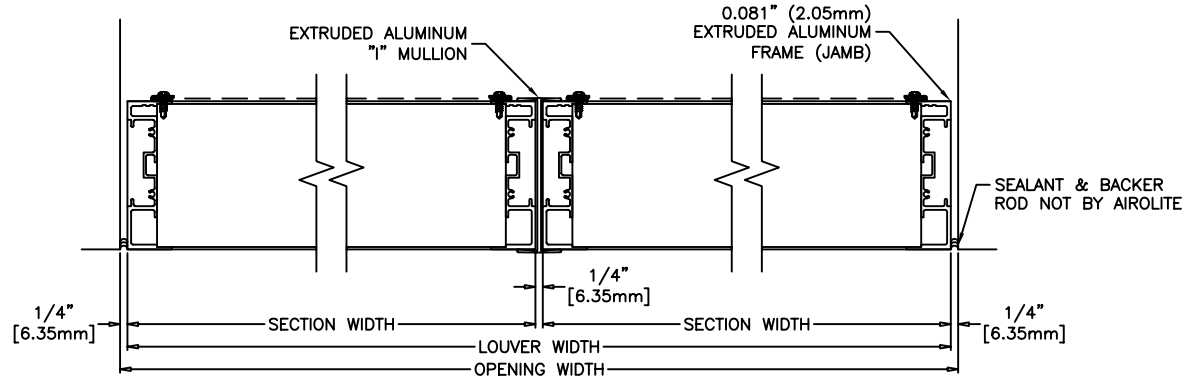
VISIBLE VERTICAL MULLION
