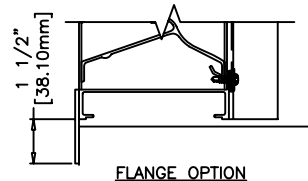
FLANGE OPTION
