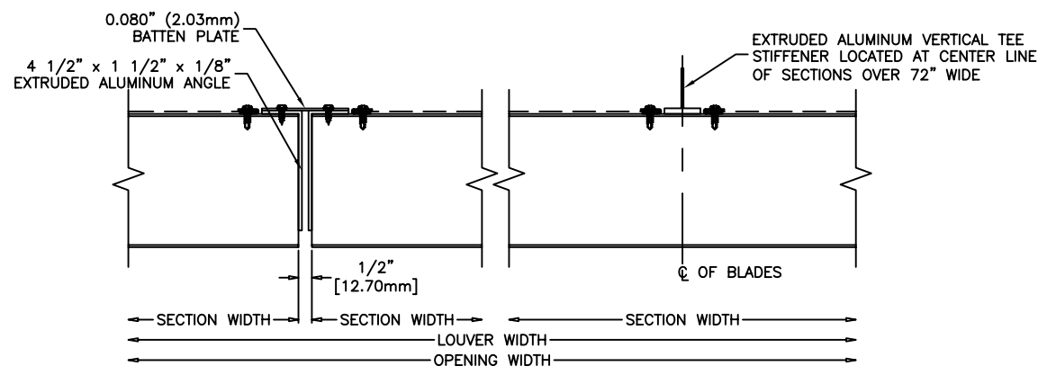
CONCEALED VERTICAL MULLION
