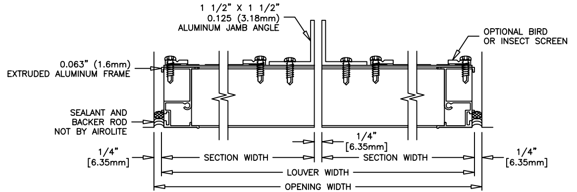
CONCEALED VERTICAL MULLION
