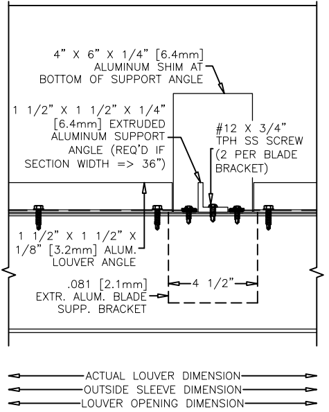
D SUPPORT DETAIL (OPENING HEIGHT \leq 96 \frac{25}{32} " )
