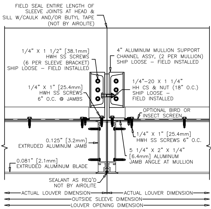
E MULLION DETAIL (OPENING HEIGHT \leq 96 \frac{25}{32} " )
