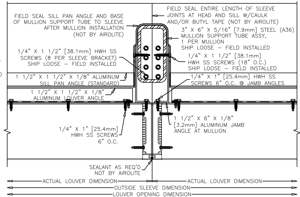
E1 MULLION DETAIL (OPENING HEIGHT > 96 25/32" - ≤ 144 25/32")
