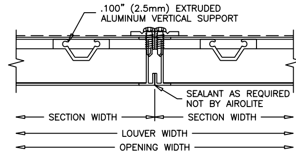
VISIBLE VERTICAL MULLION
