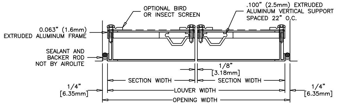
CONCEALED VERTICAL MULLION
