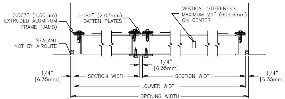
VISIBLE VERTICAL MULLION W/BATTEN PLATES
