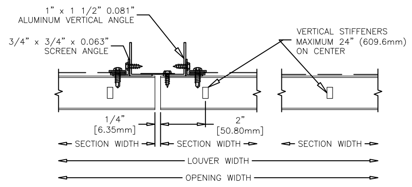
CONCEALED VERTICAL MULLION
