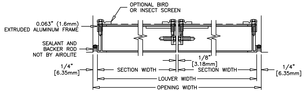
CONCEALED VERTICAL MULLION
