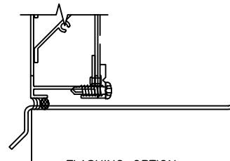
FLASHING OPTION
