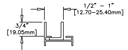
GLAZING FRAME
