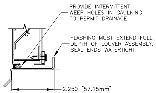
FLASHING OPTION
