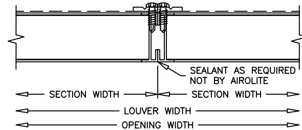
VISIBLE VERTICAL MULLION
