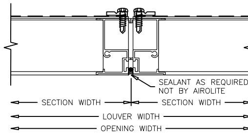
VISIBLE VERTICAL MULLION
