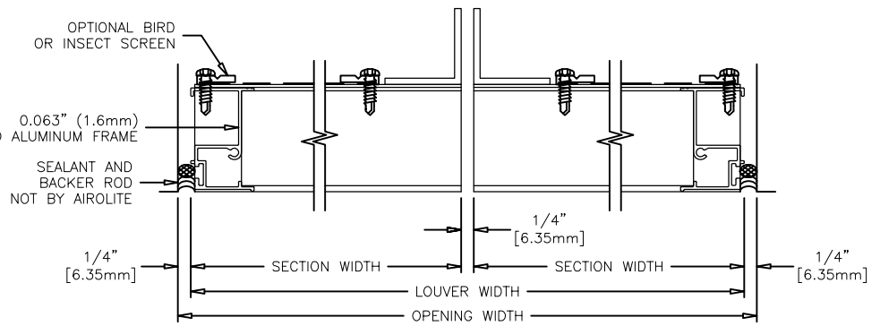
CONCEALED VERTICAL MULLION
