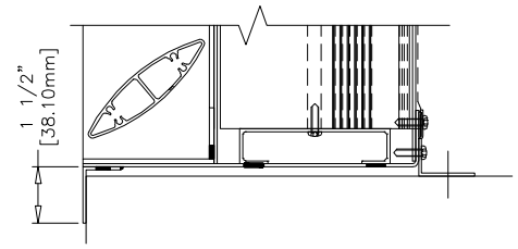
FLANGE OPTION
