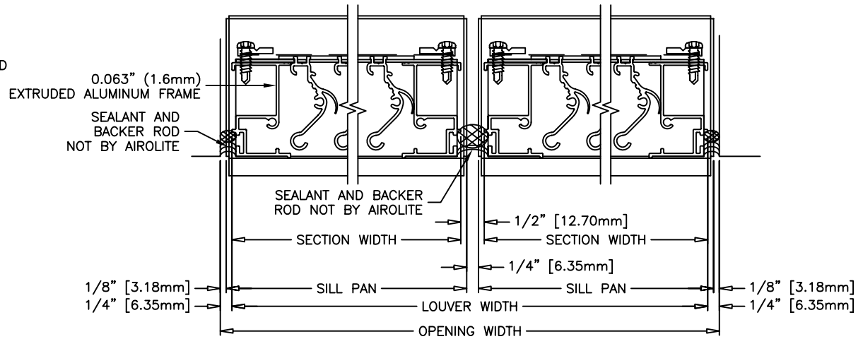
VISIBLE VERTICAL MULLION
