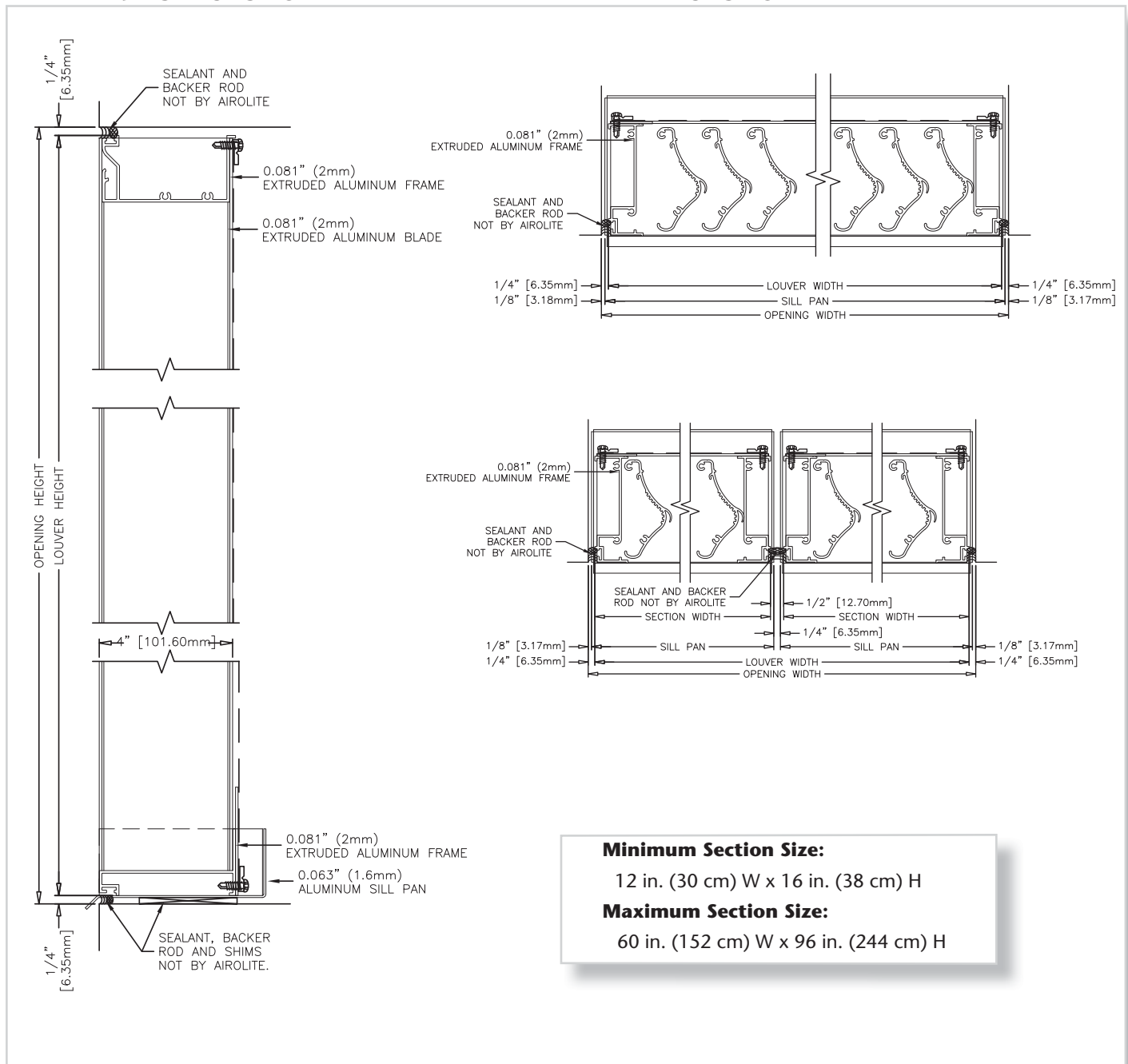
VERTICAL SECTION DETAIL
