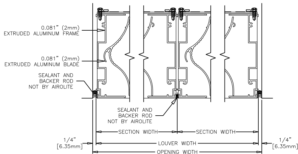
VISIBLE VERTICAL MULLION
