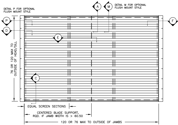
AFG801 JAMB MOUNT – ELEVATION
