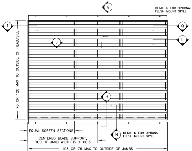
AFG801 HEAD/SILL MOUNT – ELEVATION
