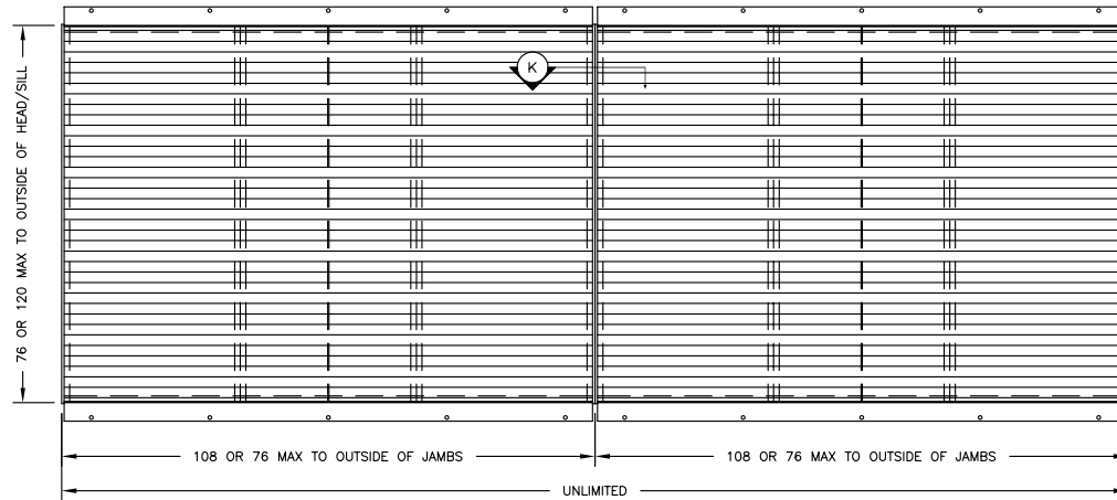
AFG801 HEAD/SILL MOUNT – MULLED ELEVATION
