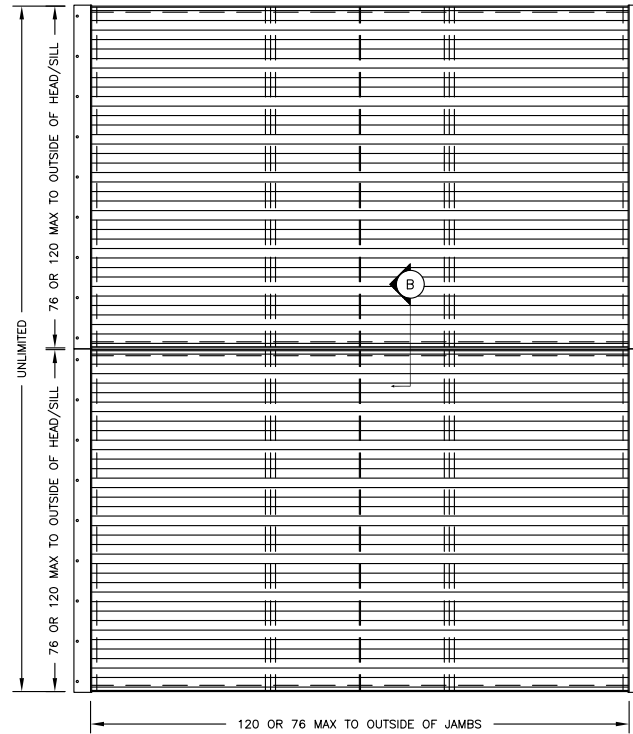
AFG801 HEAD/SILL MOUNT – MULLED ELEVATION
