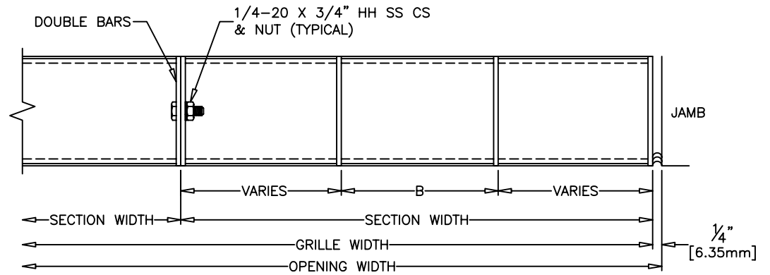
VERTICAL MULLION
